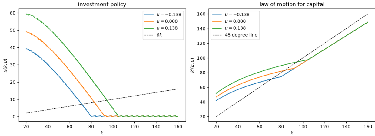
Fig. 114.1: Investment policy and law of motion
