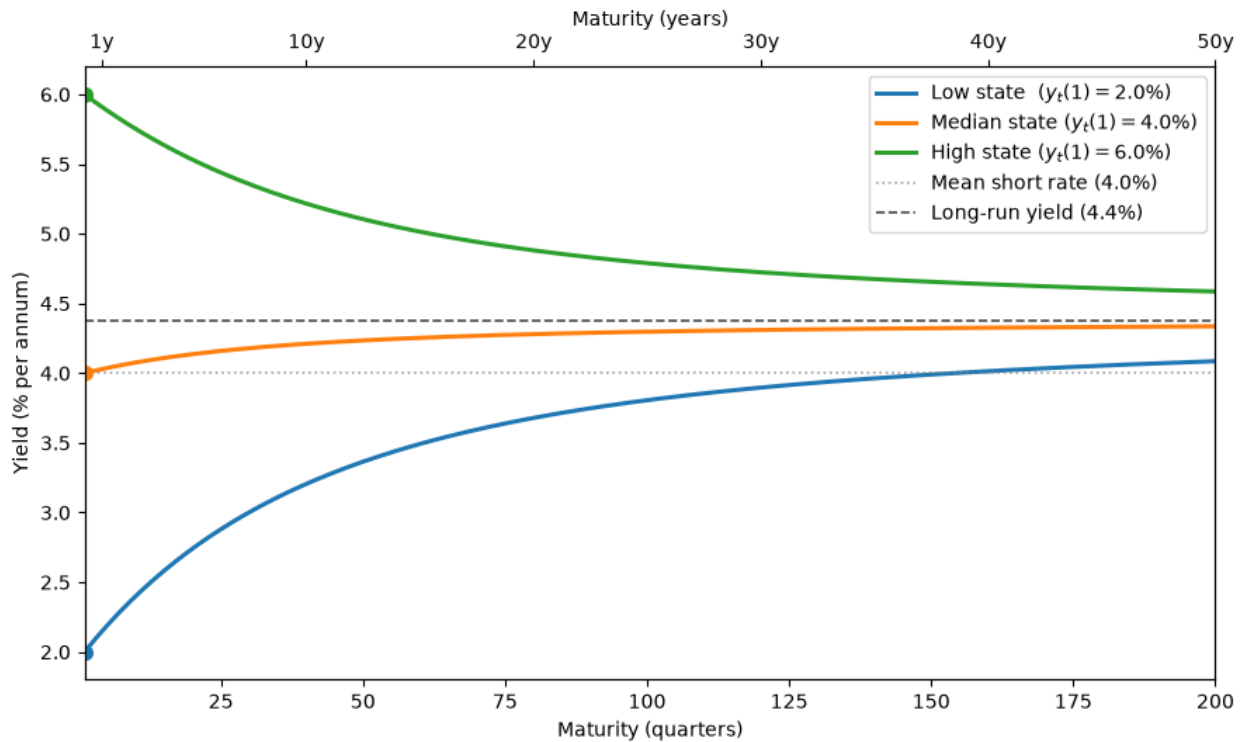
Fig. 133.1: Yield curves under the one-factor affine model
