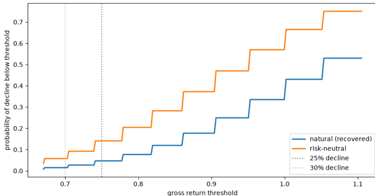
Fig. 134.1: Tail probabilities under the recovered natural and risk-neutral measures
