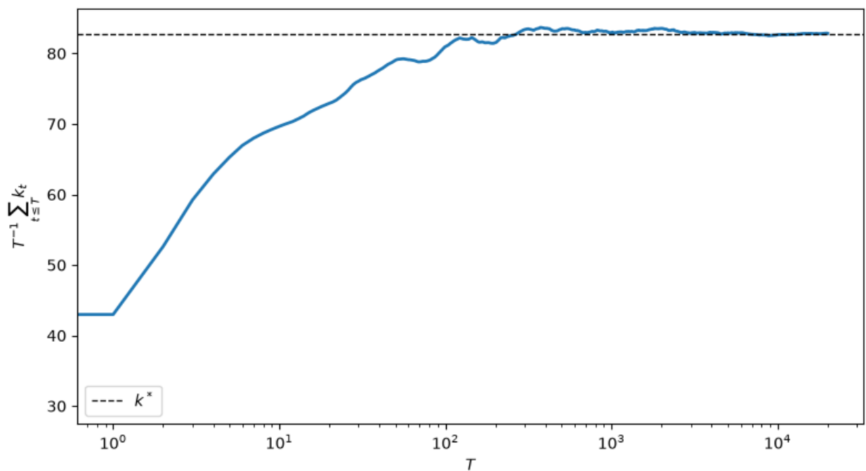
Fig. 114.5: Time average of capital
