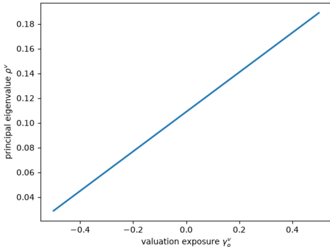
Fig. 135.5: Changing valuation functionals
