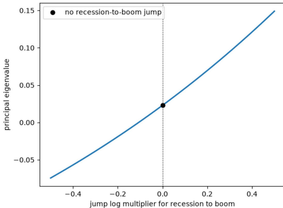
Fig. 135.2: Jumps and the long-run growth rate, holding the boom-to-recession log multiplier fixed
