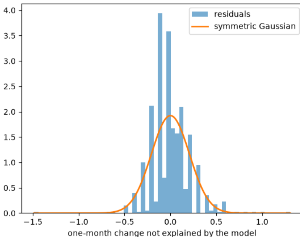
Fig. 140.4: Model residuals are right-skewed
