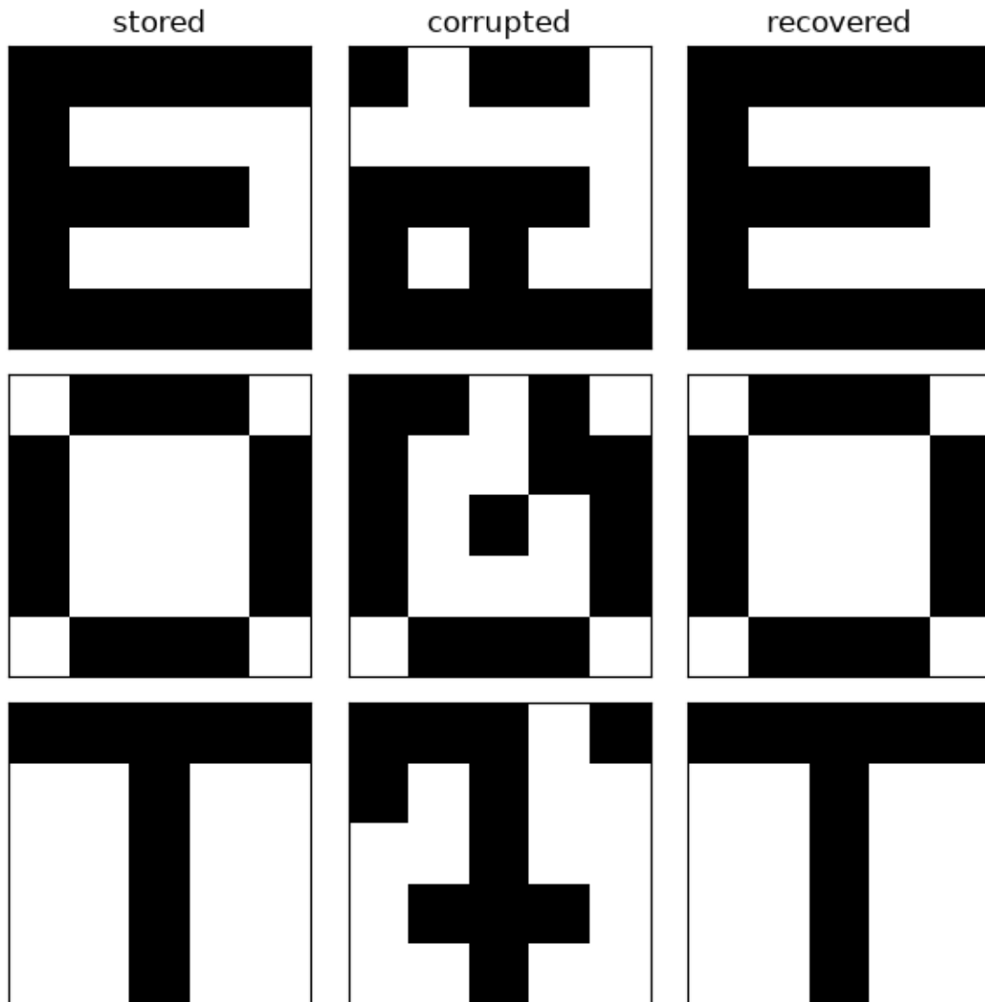
Fig. 93.2: Hopfield recall of letters from corrupted inputs
