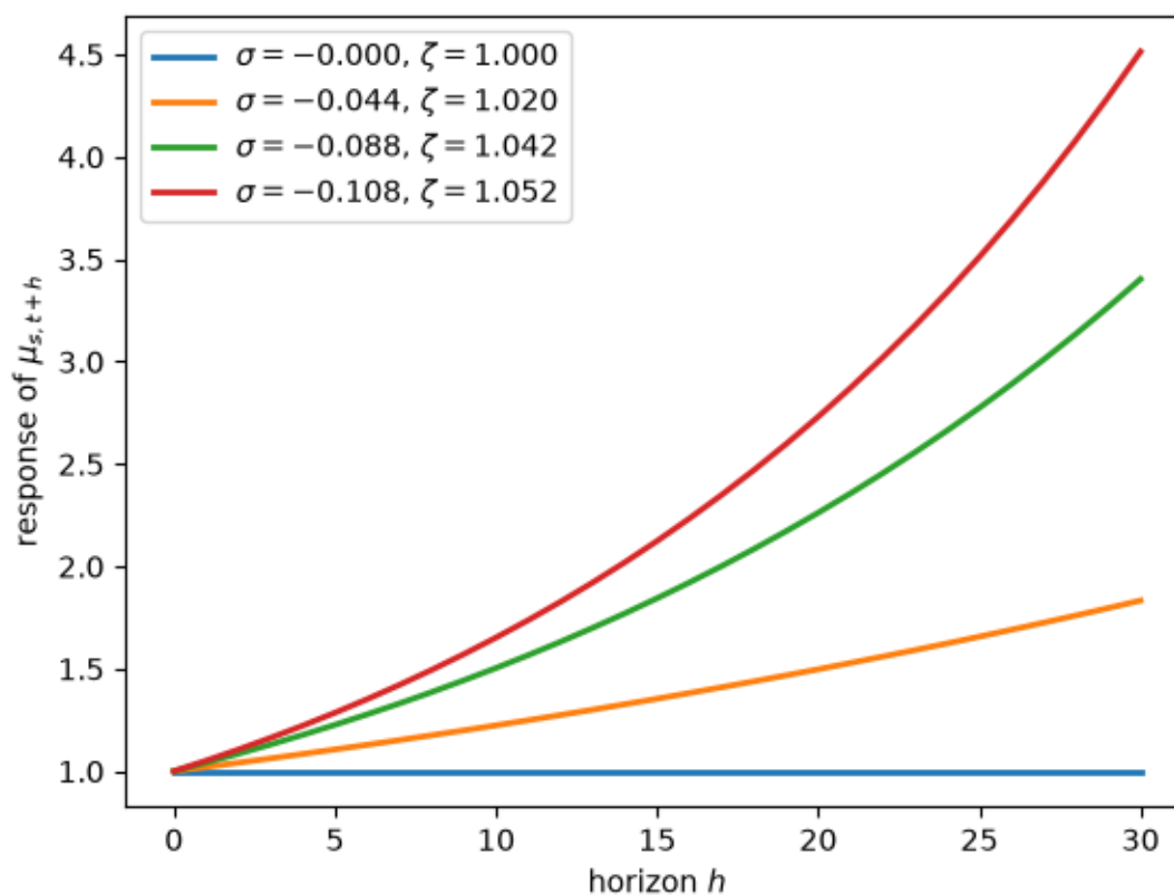
Fig. 86.2: Worst-case impulse response of marginal utility. The approximating model has a unit root; the worst-case model is increasingly explosive as \sigma falls toward the breakdown point \underline{\sigma} .
