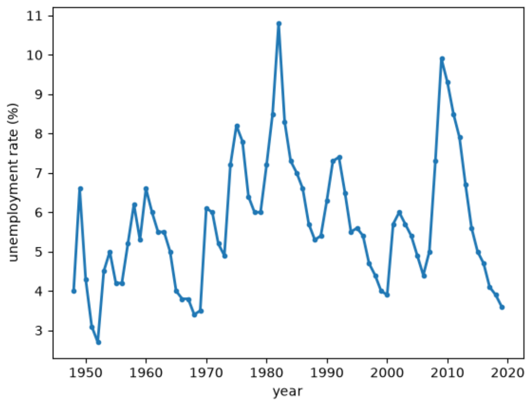
Fig. 141.1: Annual US unemployment
