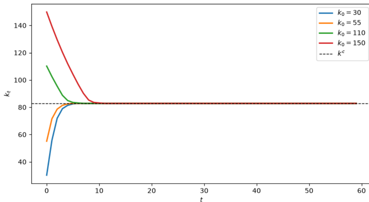
Fig. 114.2: Capital paths under IID demand
