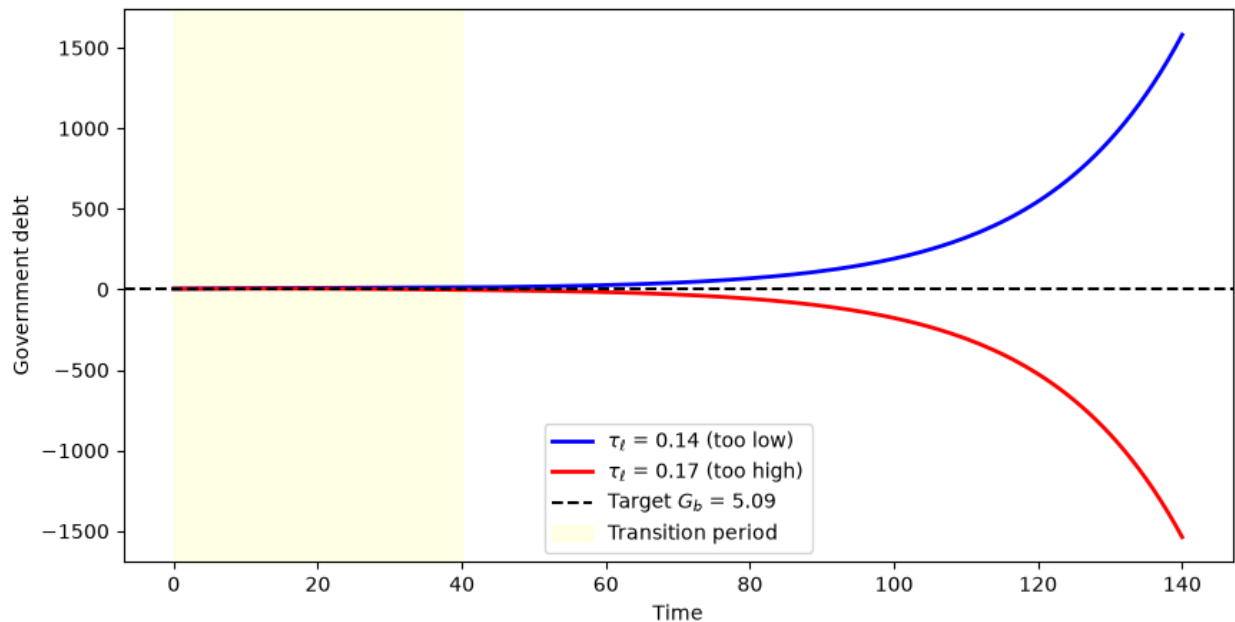
Fig. 123.5: Shooting method for finding the transition tax rate
