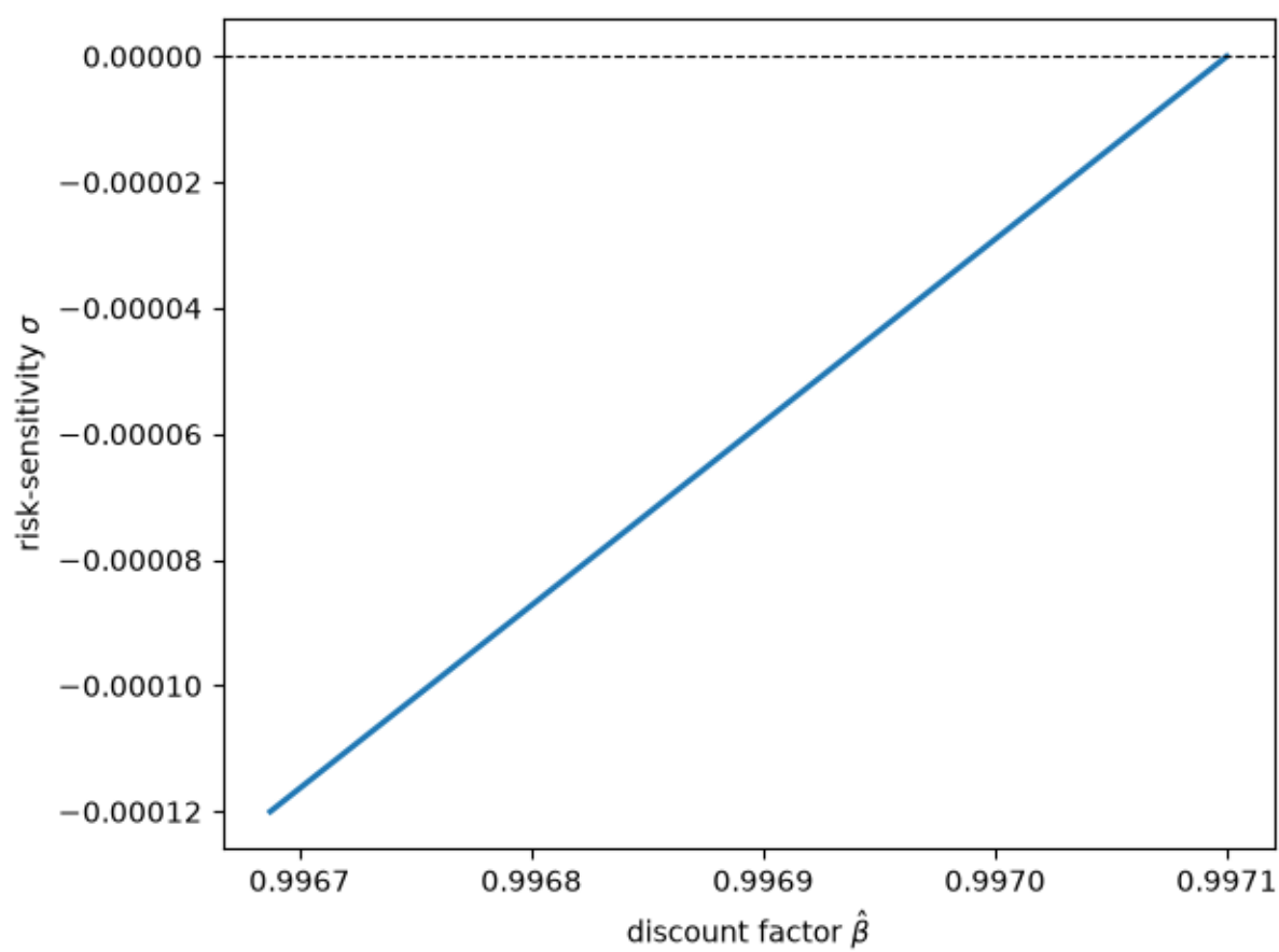
Fig. 81.2: Equivalent (\sigma, \hat{\beta}) pairs
