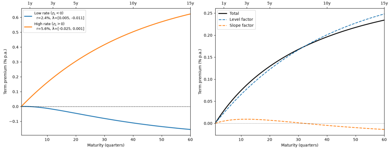
Fig. 133.4: Term premiums and factor decomposition under the two-factor model
