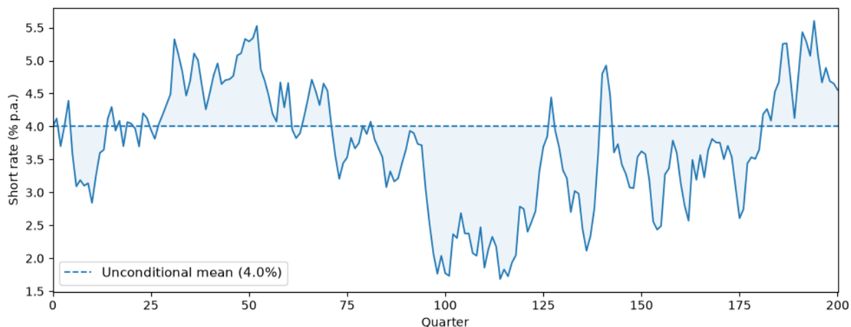
Fig. 133.2: Simulated short rate path
