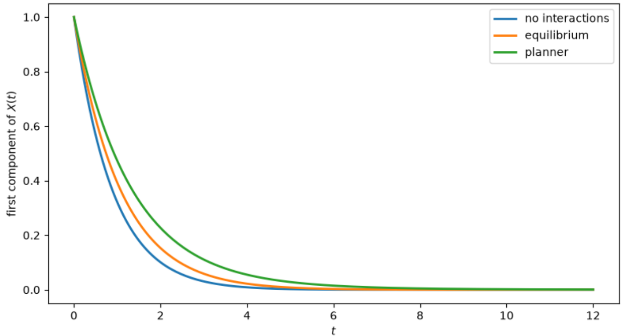
Fig. 124.3: Path of the aggregate state
