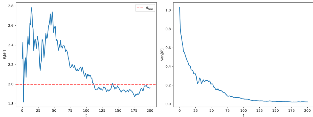
Fig. 131.2: posterior mean and variance over time
