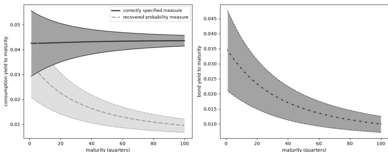
Fig. 136.2: Yield implications of using the recovered probability measure as beliefs. Dashed consumption-yield bands use payoff forecasts under the recovered probability measure with prices fixed; bond yields are unchanged because the zero-coupon payoff has no forecast term.
