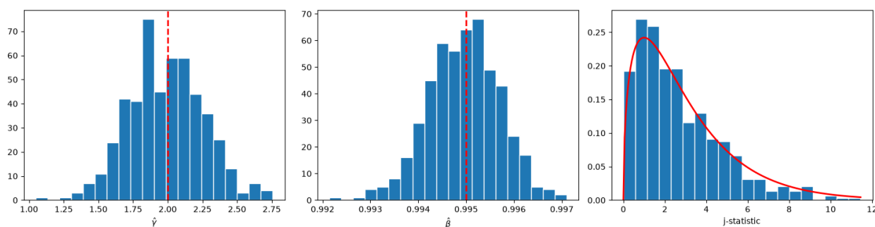
Fig. 127.2: Monte Carlo GMM sampling distributions
