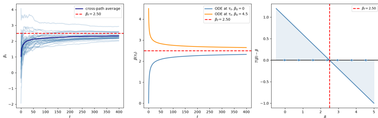
Fig. 132.1: Bray learning dynamics
