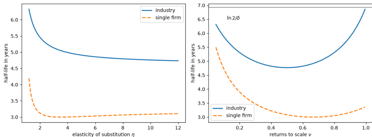
Fig. 124.1: Half-lives of industry and firm capital
