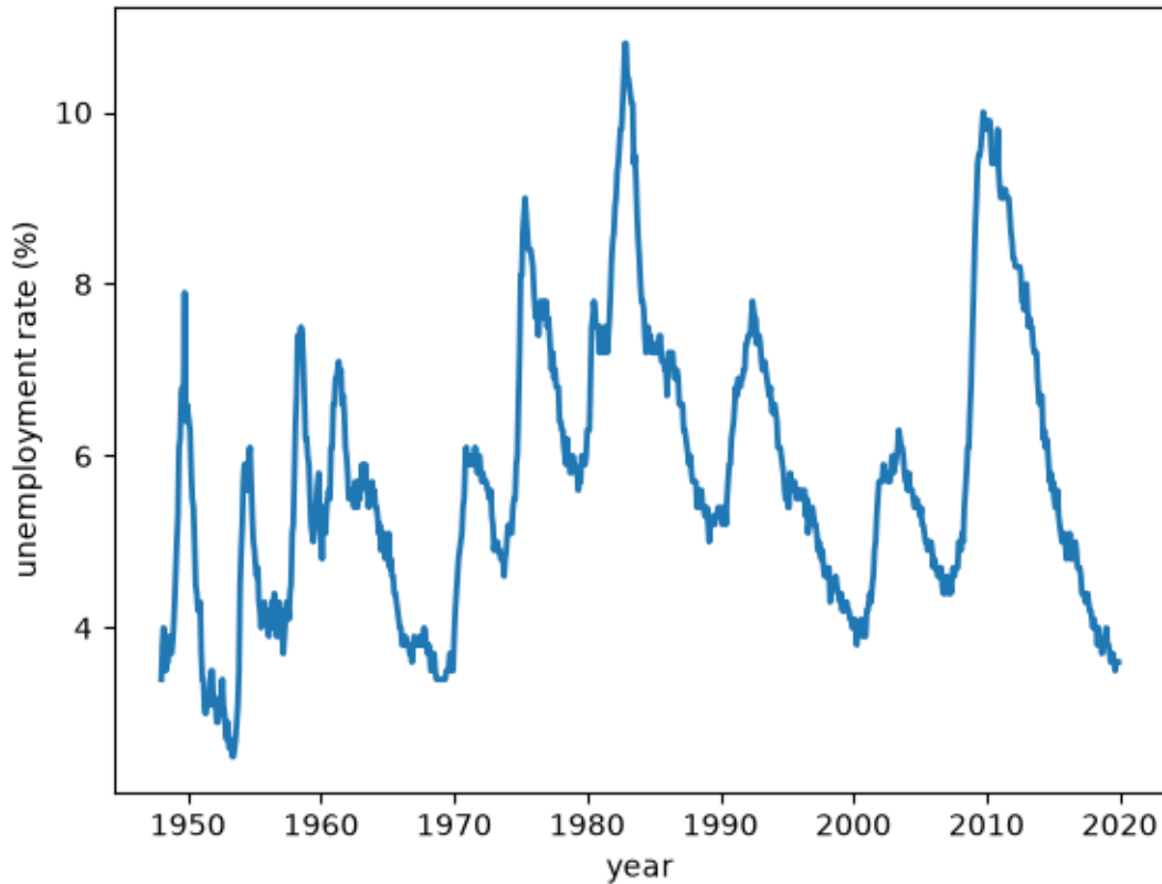
Fig. 140.1: US monthly unemployment rate, 1948–2019
