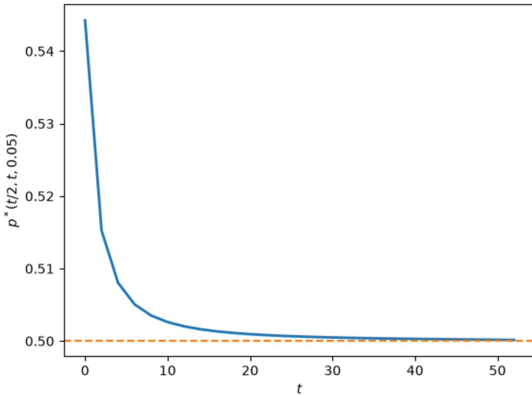
Fig. 130.2: Normalized price against time
