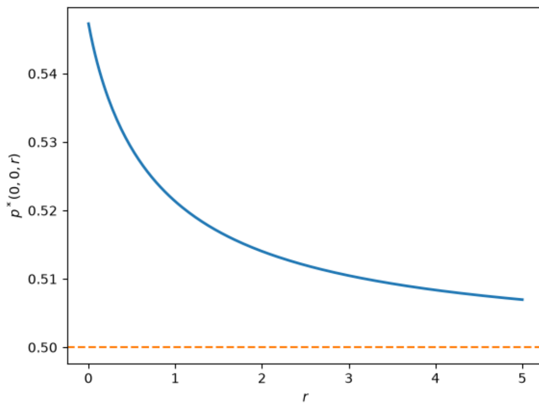
Fig. 130.1: Normalized price against interest rate
