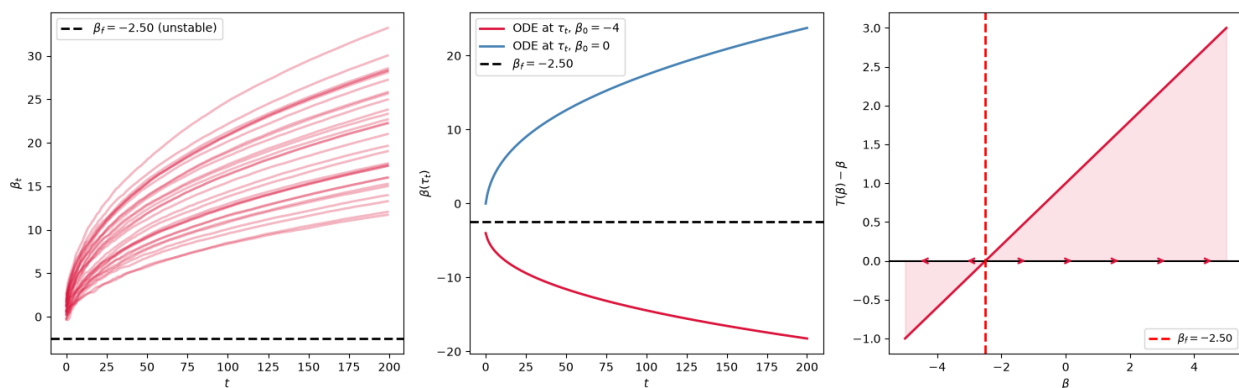
Fig. 132.2: Unstable Bray dynamics
