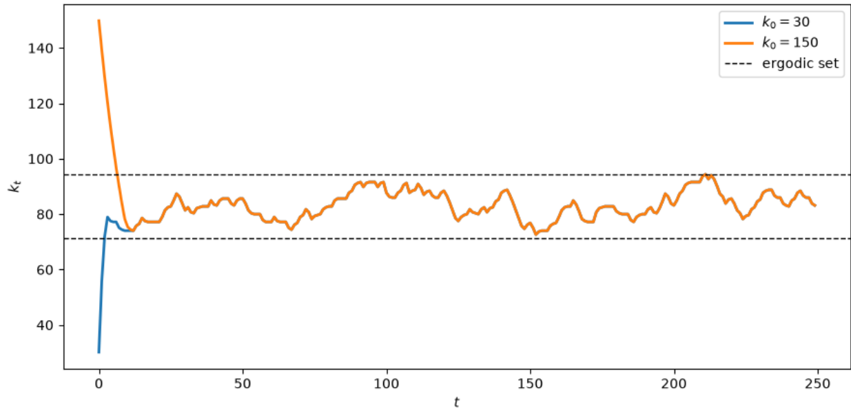
Fig. 114.3: Capital paths entering the ergodic set
