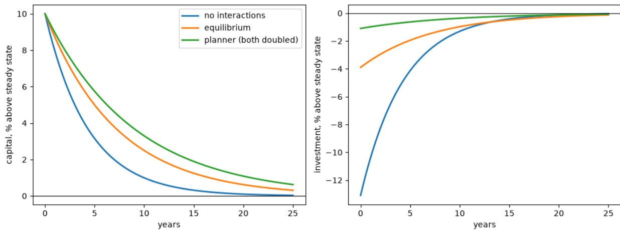
Fig. 124.2: Transition paths of capital and investment
