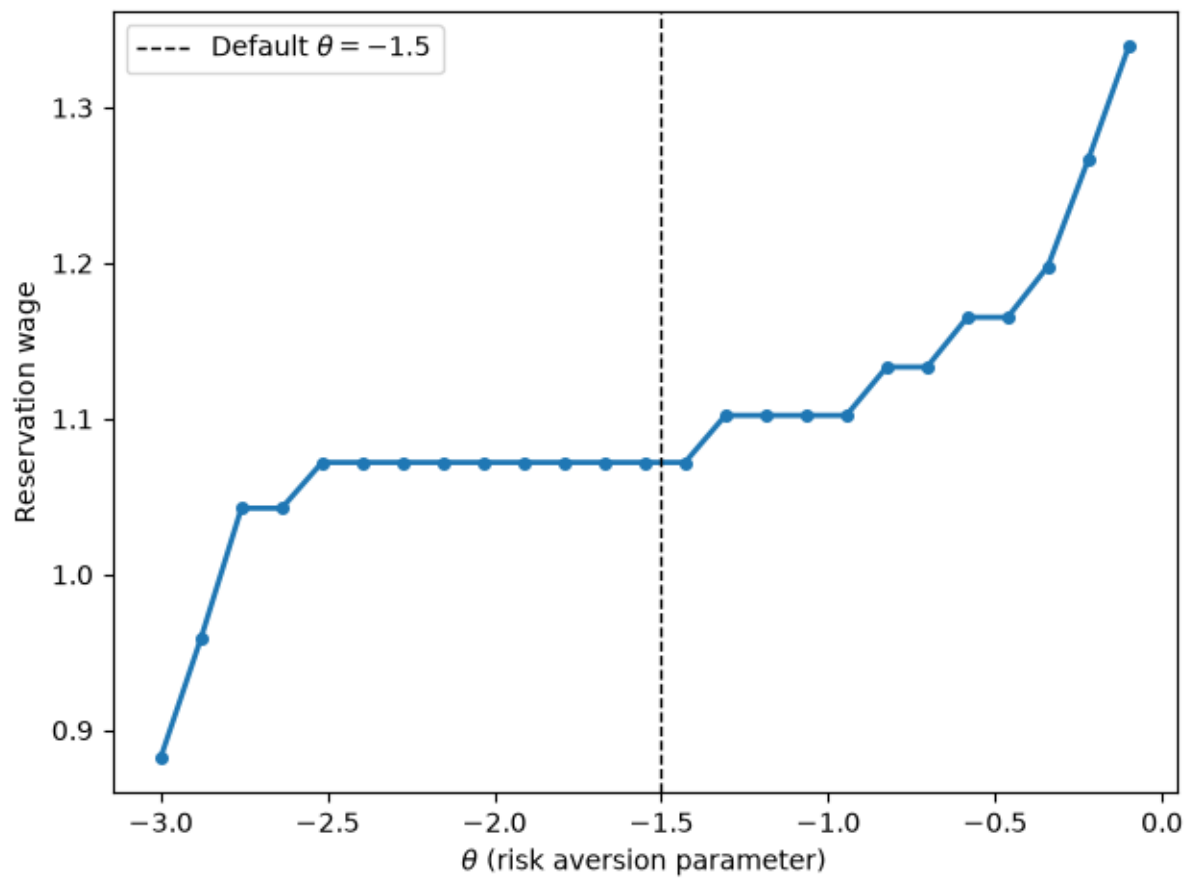
Fig. 57.3: Reservation wage against risk aversion
