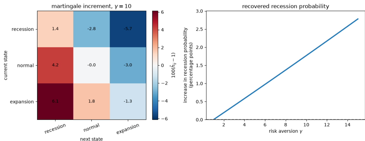
Fig. 136.1: Recursive utility generates a nonconstant martingale increment.
