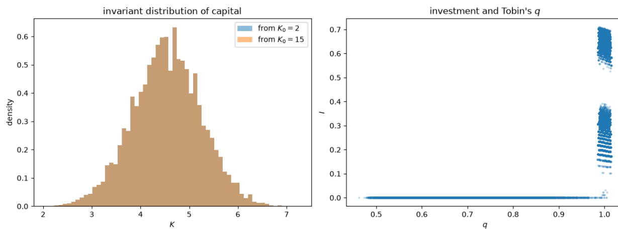
Fig. 115.2: Invariant distribution and investment against q
