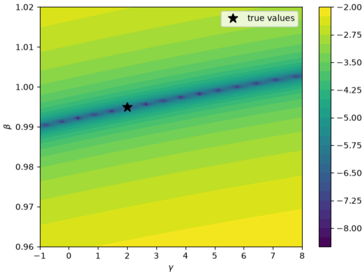
Fig. 127.1: GMM objective contour surface (simulated data)
