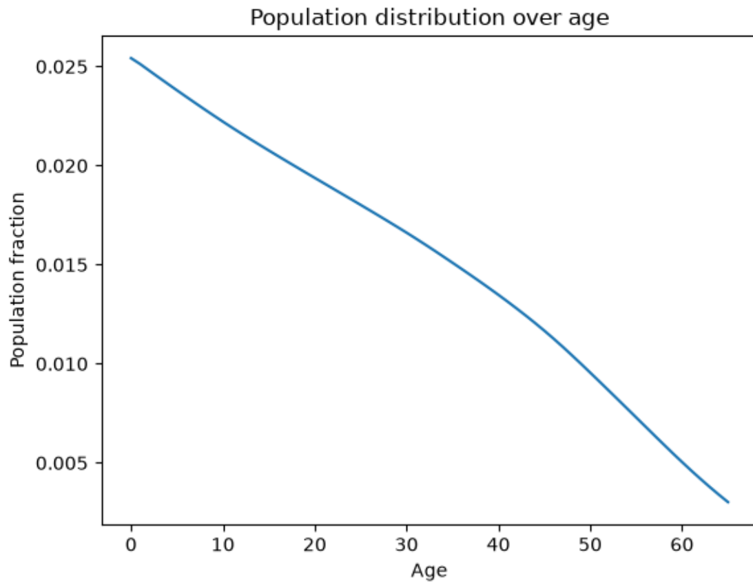
Fig. 123.3: Stationary population distribution over age
