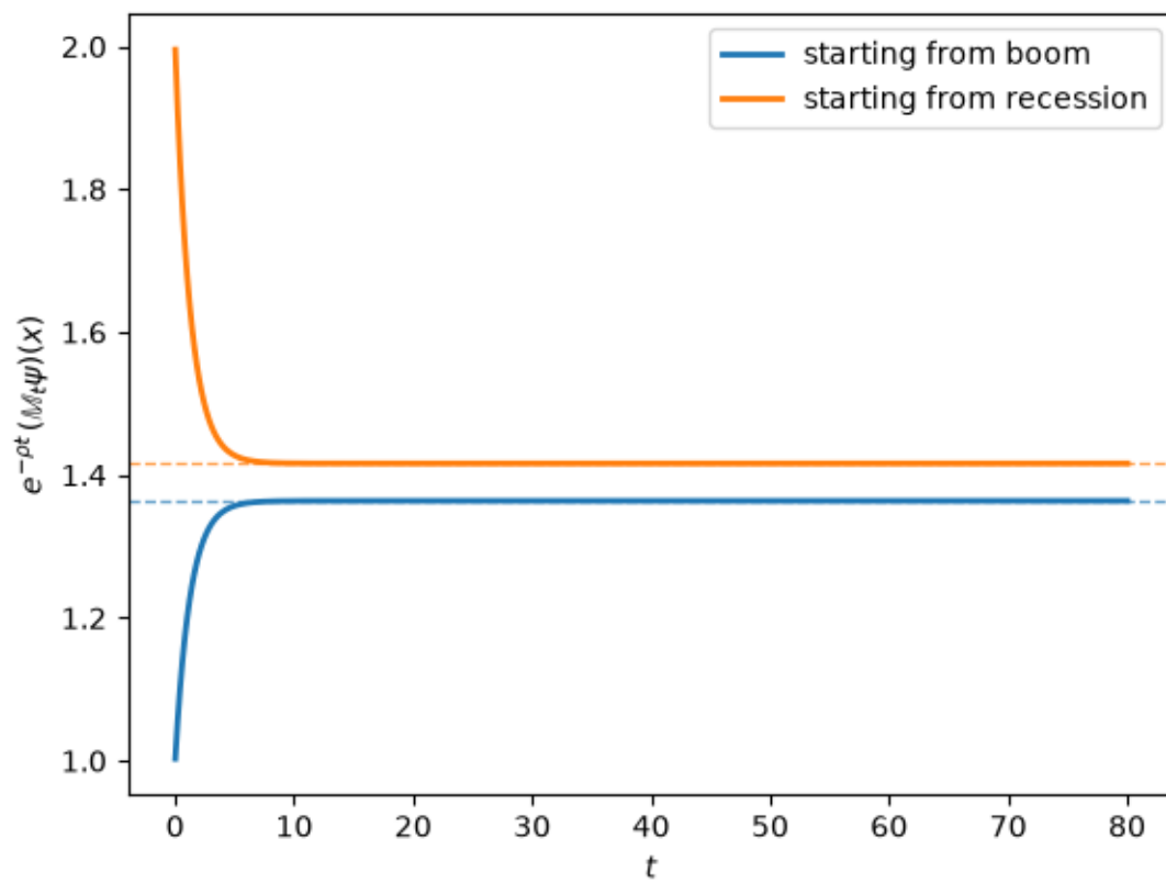
Fig. 135.1: Convergence of the rescaled semigroup to its long-run limit
