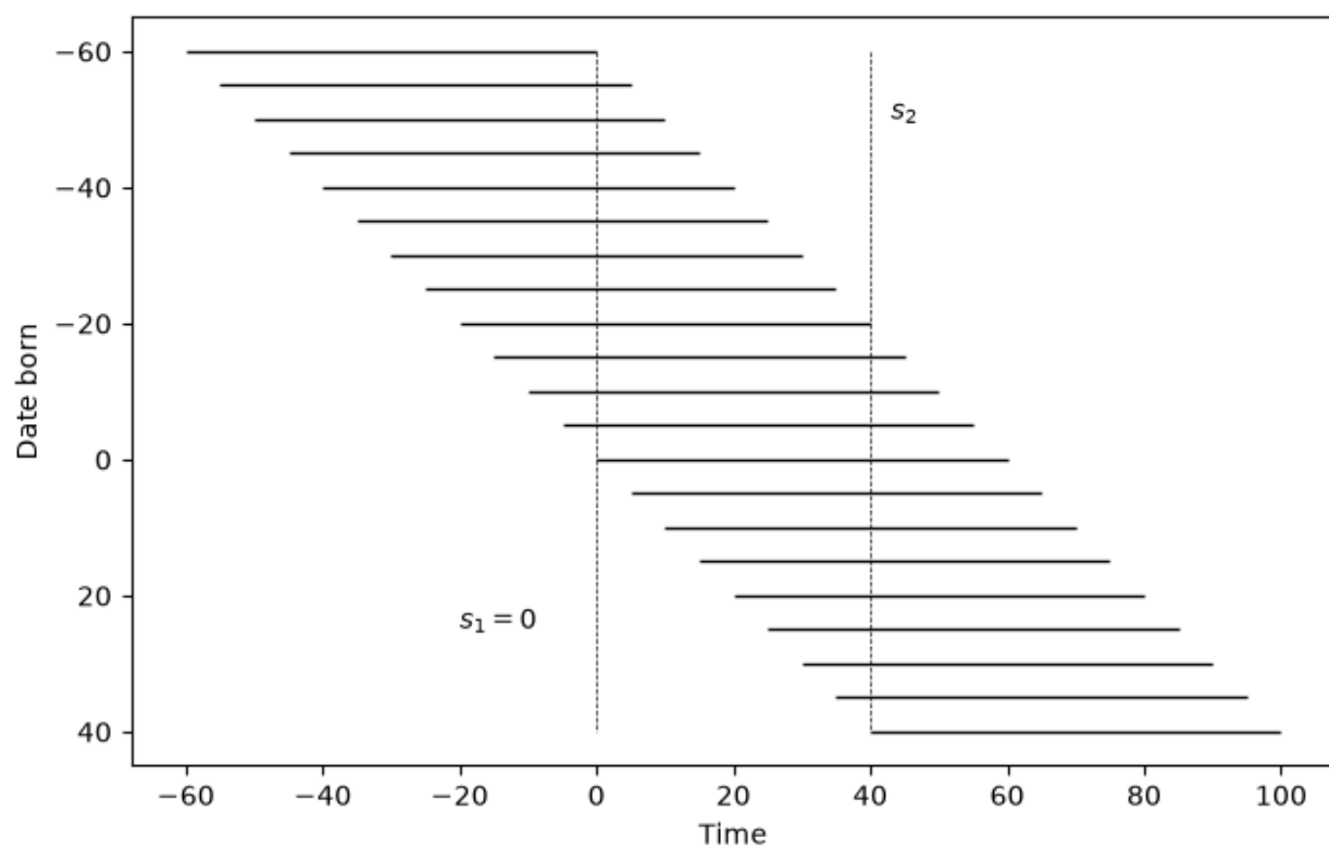
Fig. 123.1: Age-time diagram for overlapping generations
