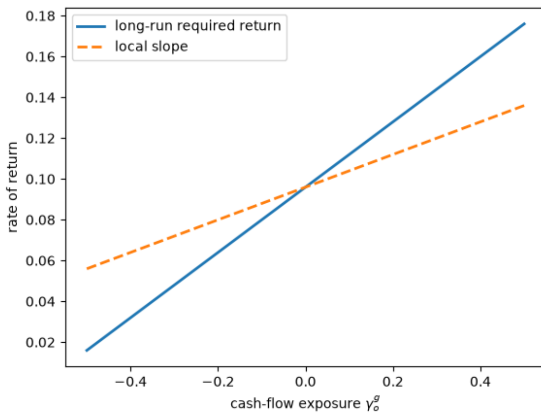
Fig. 135.6: Local and long-run pricing of persistent growth risk
