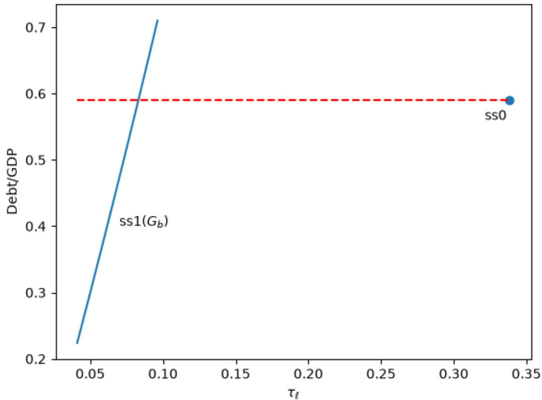
Fig. 123.4: Debt-to-GDP ratio as a function of the labor tax rate
