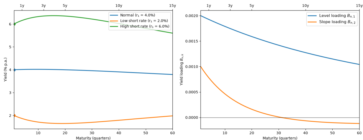
Fig. 133.3: Yield curves and factor loadings under the two-factor model
