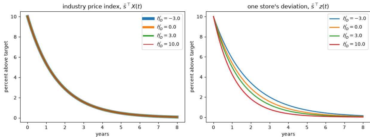
Fig. 124.4: Industry and store price paths
