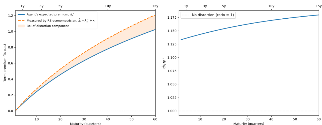
Fig. 133.5: Subjective vs. measured term premiums and overstatement ratio
