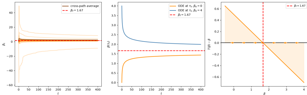
Fig. 132.3: Bray-Savin learning dynamics
