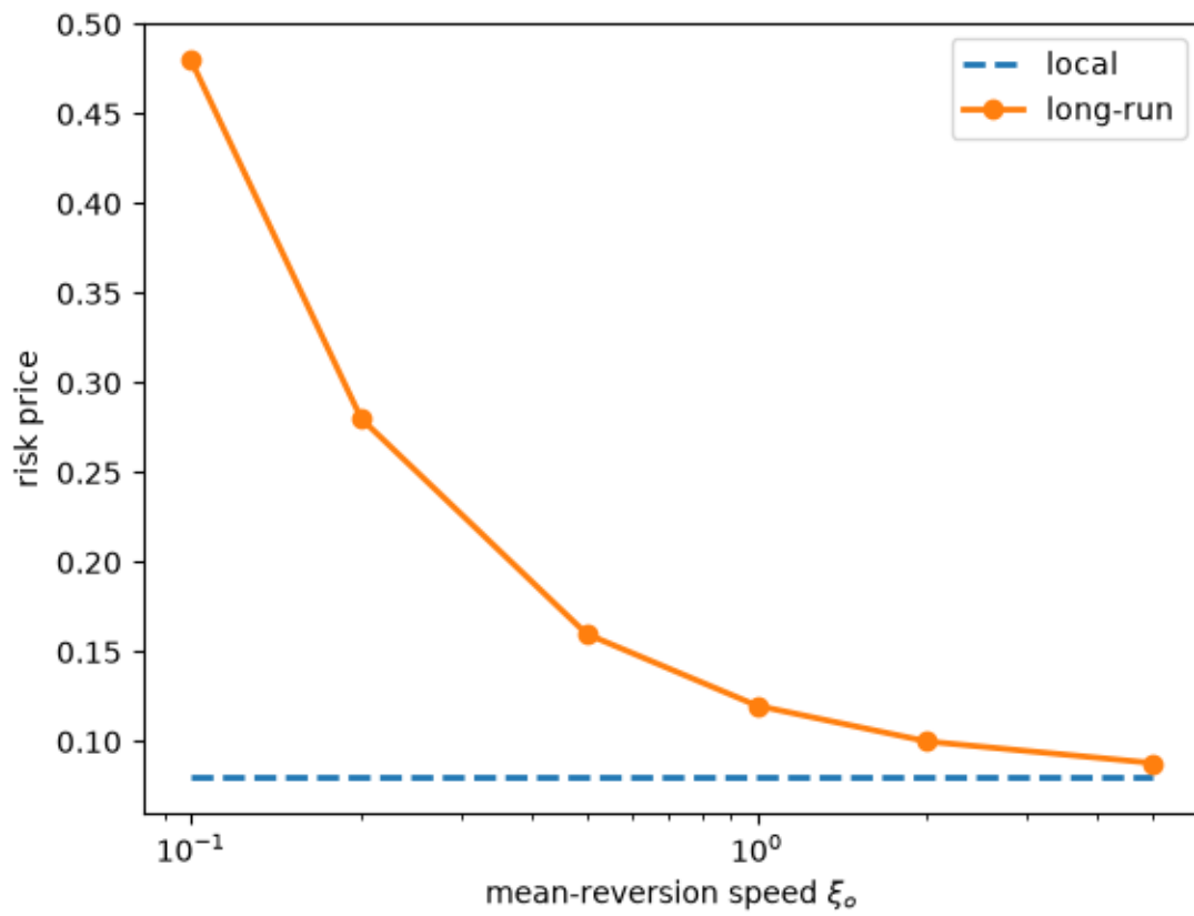
Fig. 135.4: Persistence and long-run risk prices
