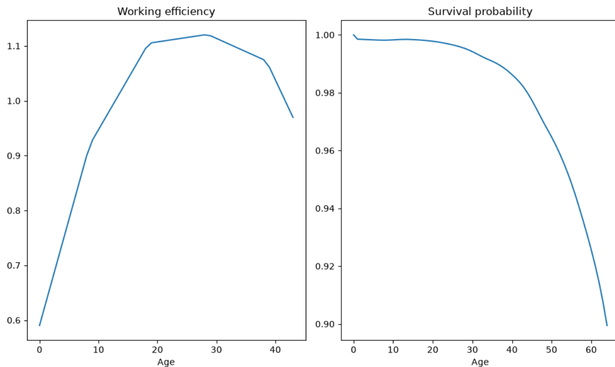
Fig. 123.2: Age-efficiency profile and survival probabilities
