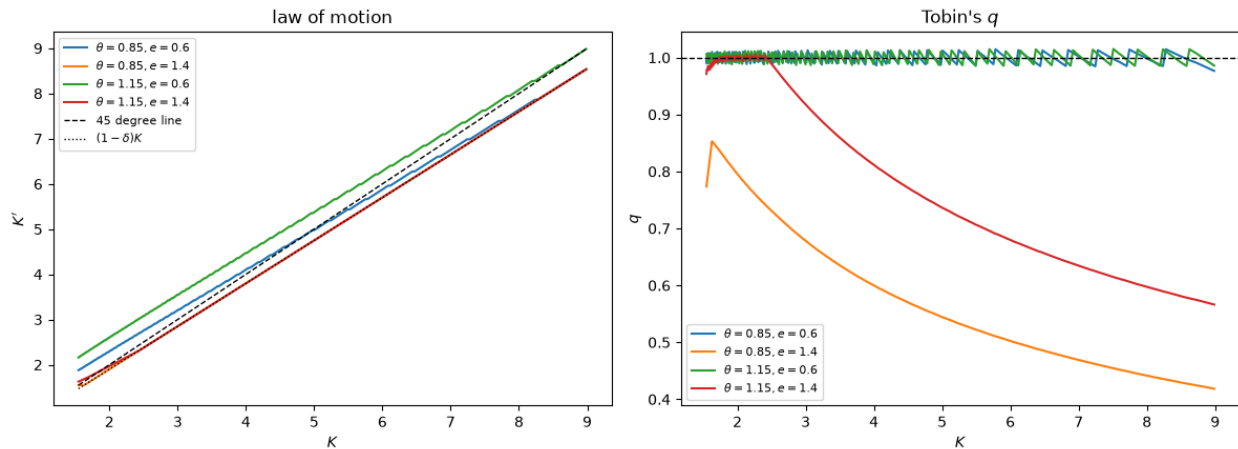
Fig. 115.1: Law of motion and Tobin's q
