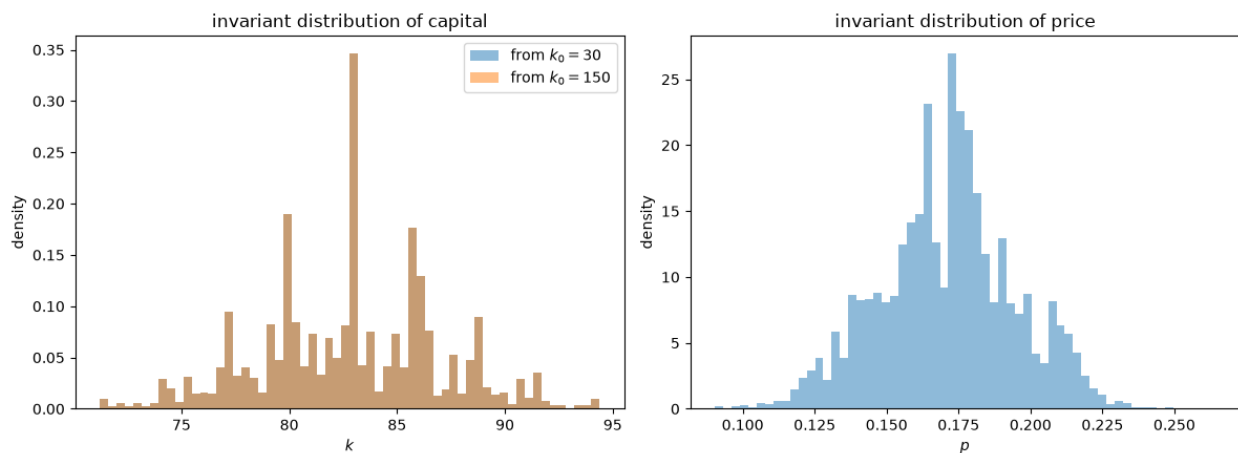
Fig. 114.4: Invariant distributions of capital and price
