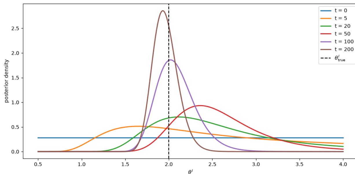
Fig. 131.1: posterior density over \theta^I at selected dates
