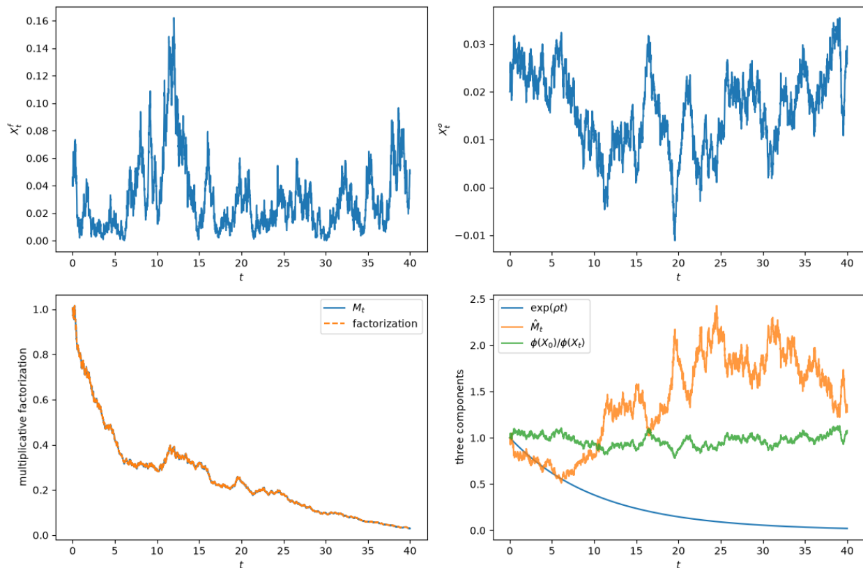
Fig. 135.3: Affine state paths and multiplicative factorization
