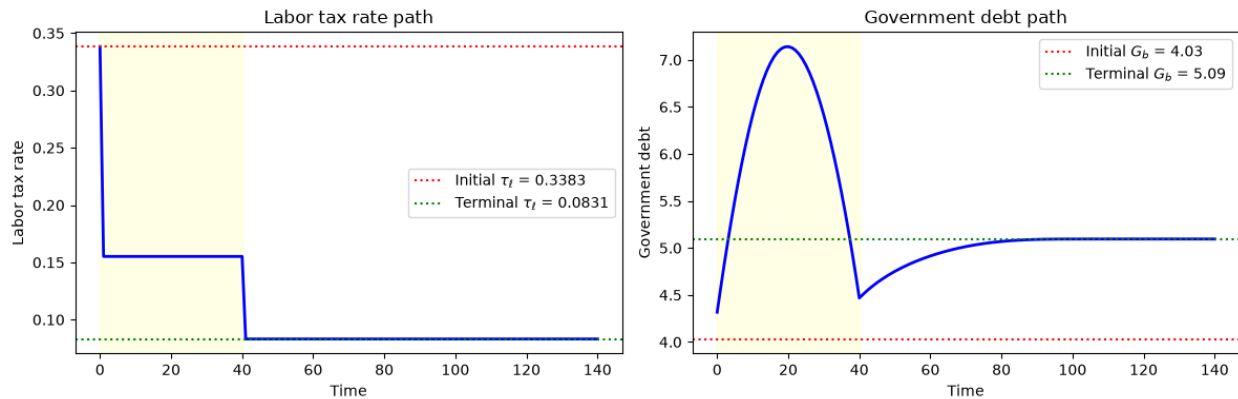
Fig. 123.6: Baseline transition path (no compensation)
