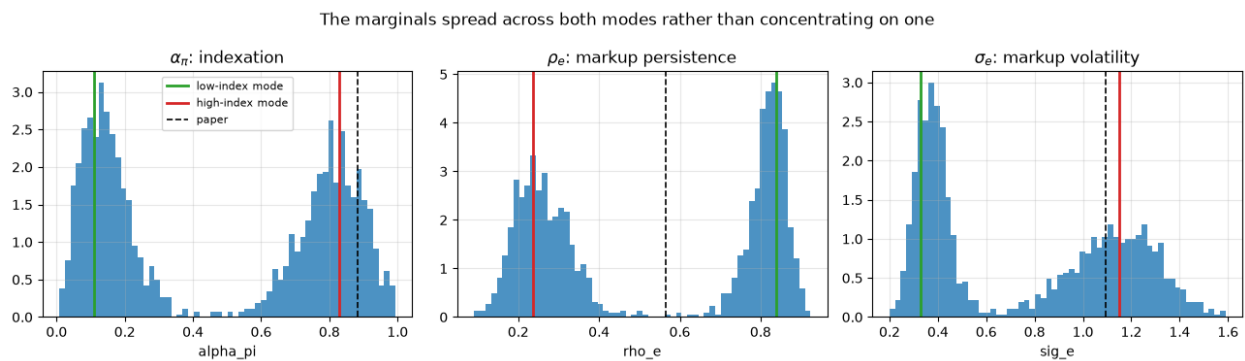
Fig. 142.1: Marginal posteriors for the parameters that separate the two modes
