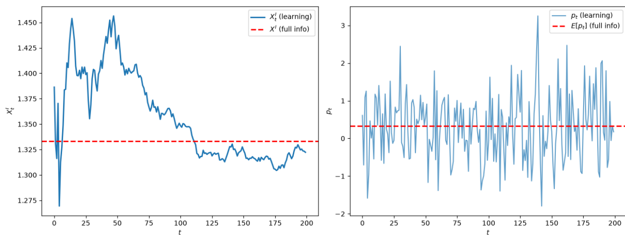
Fig. 131.3: equilibrium trade and prices over time
