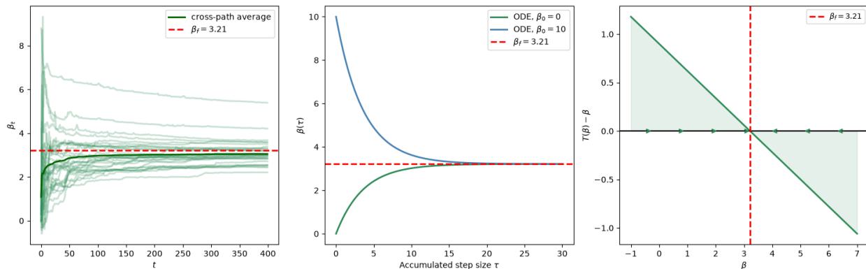
Fig. 132.4: Present-value learning dynamics
