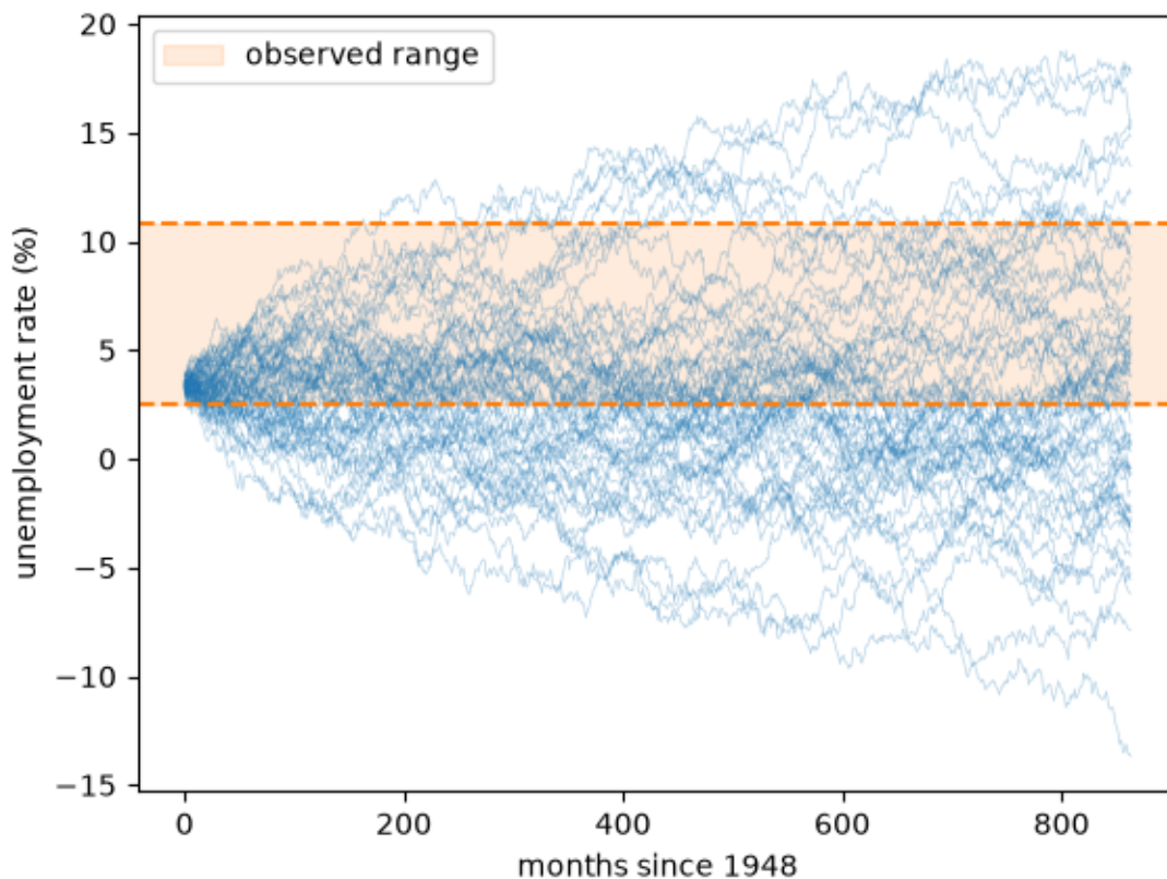
Fig. 140.2: Random walks leave the observed range
