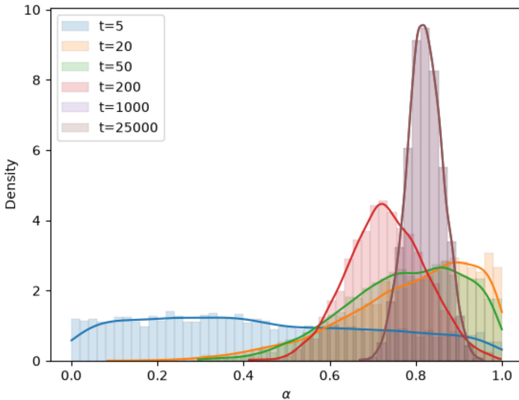
Fig. 32.6: Posterior for \alpha as t grows
