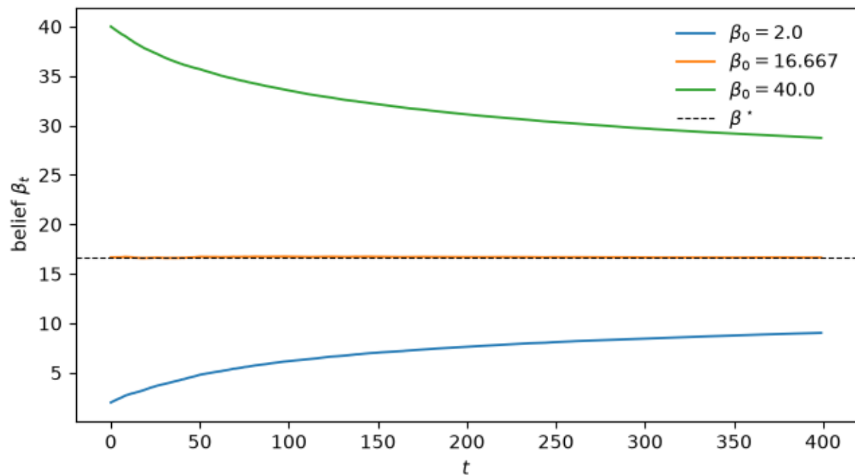
Fig. 95.1: The belief forgets its starting point
