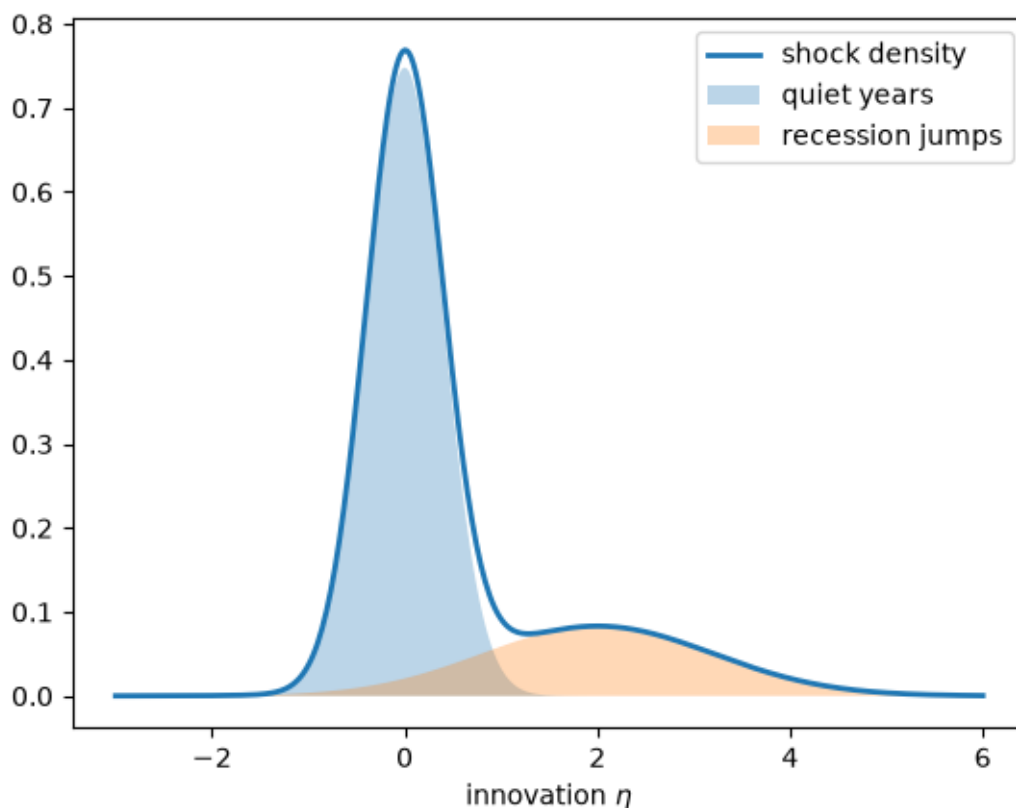
Fig. 141.2: Shock distribution as a mixture
