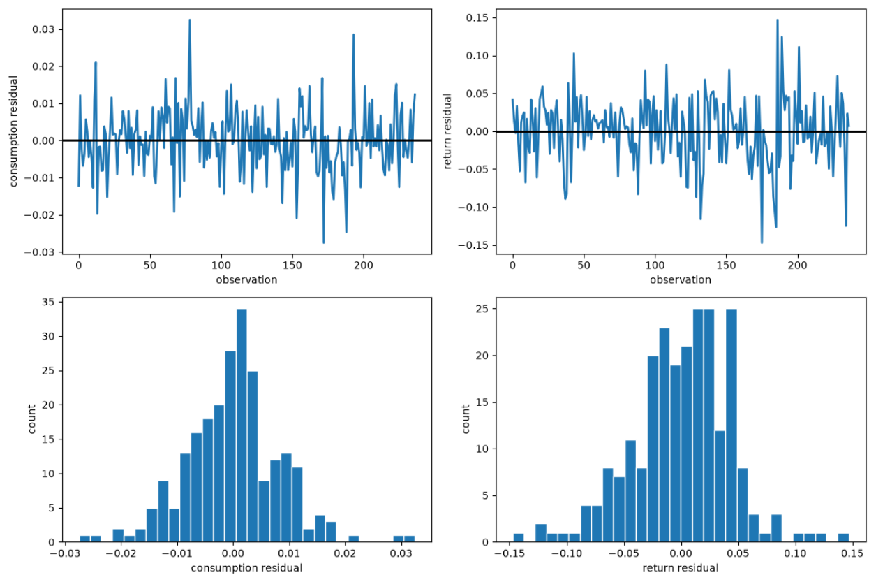
Fig. 126.1: Restricted-model residual diagnostics
