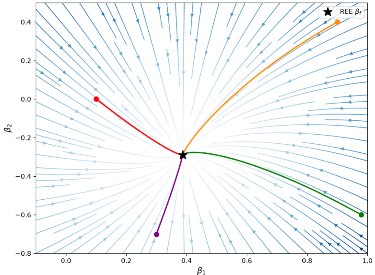
Fig. 132.5: Investment phase portrait
