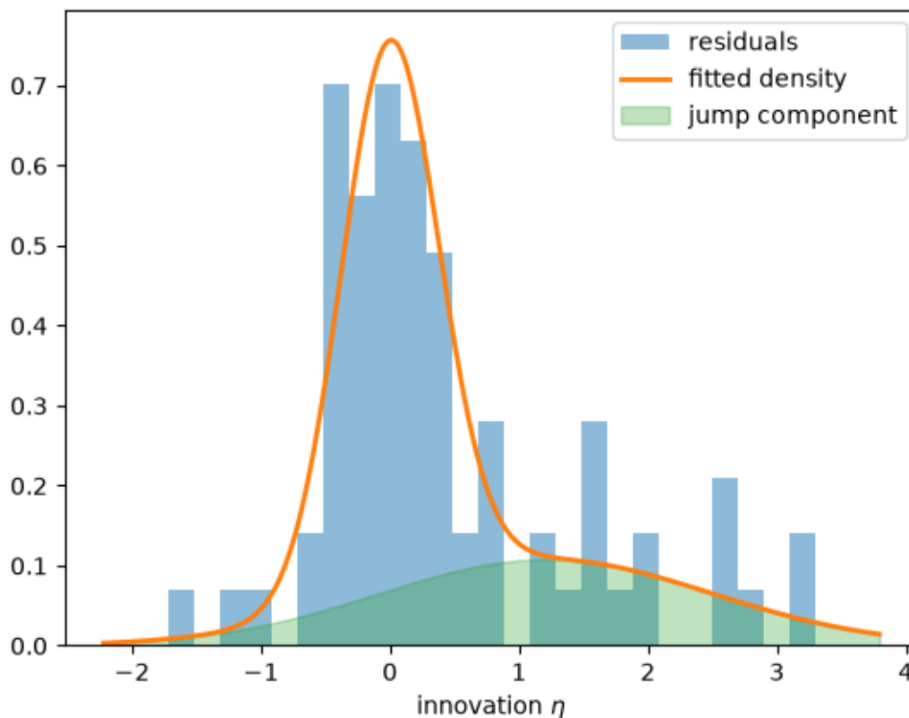
Fig. 141.3: Fitted shock density against the residuals
